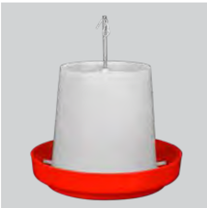
■ Manual Feeder High Density polyethylene Capacity : 4 Kgm Weight 320 gm
